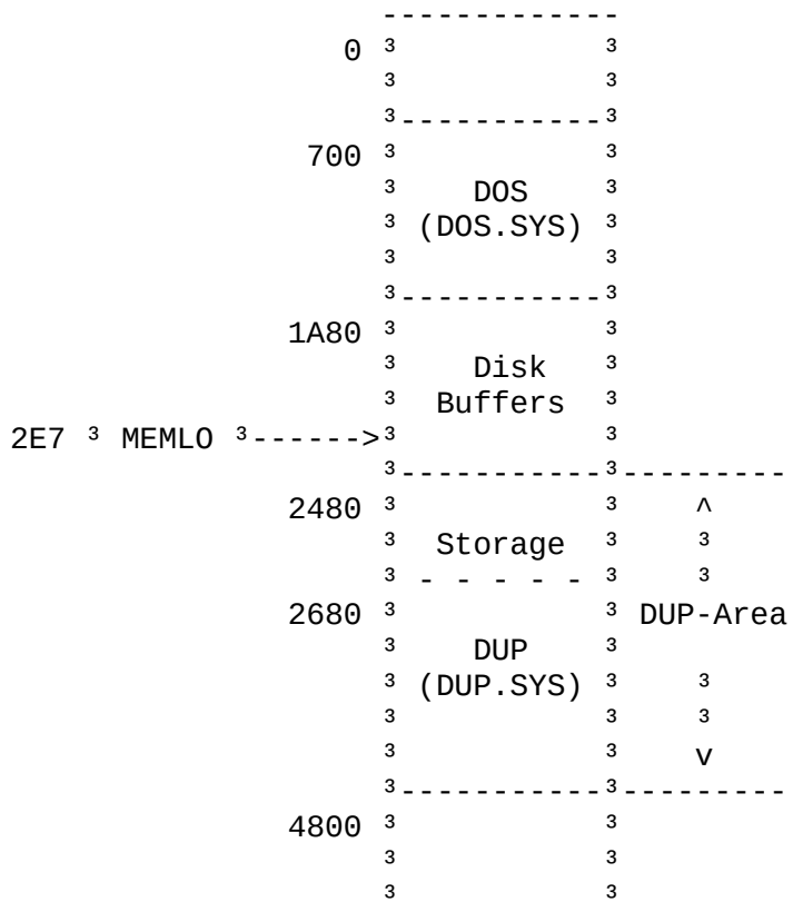
Figure 1. Memory Map of TOP-DOS.
